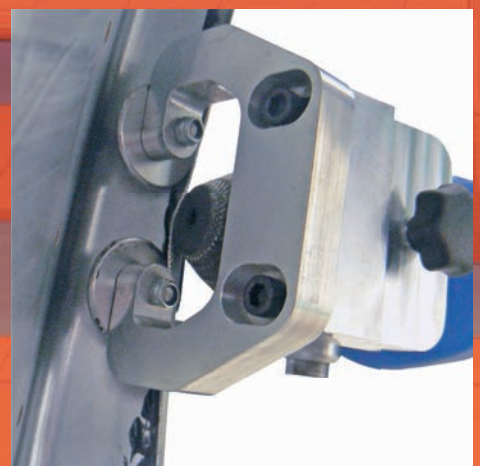
RFW 2000 with wheel house kit Art.-No. 562051 (accessory)
