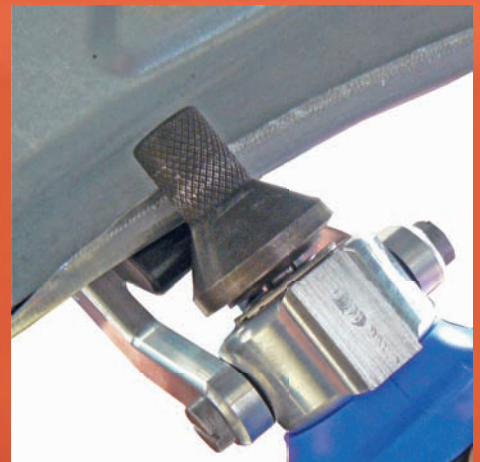
RFW 2000 with powerful planetary gearing
