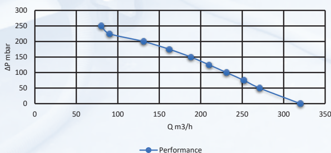
TKW3 3 kW
